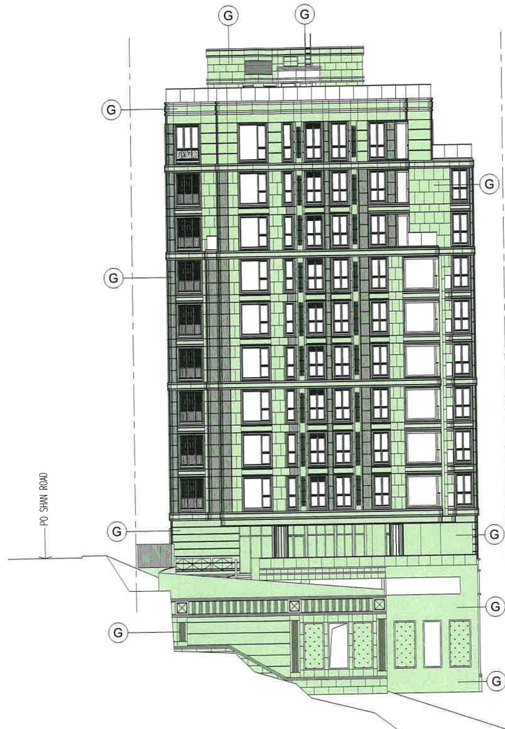
EAST ELEVATION
